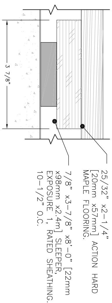
ActionProAir_WBS Section across room length
