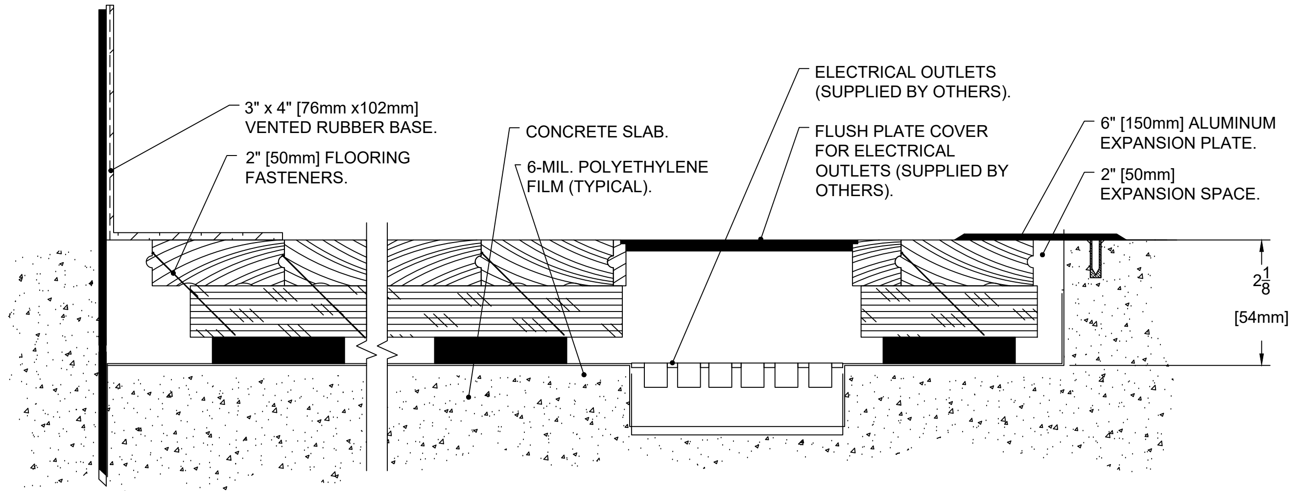
Section across room width ActionProAir WBS
